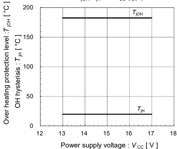
Over heating characteristics
