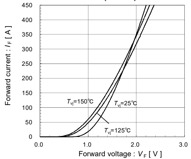
Forward current vs. Forward voltage (typ.)
