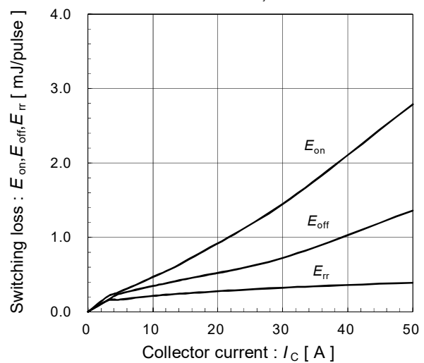
Switching loss vs. Collector current (typ.) V_{DC}=300\text{V}, V_{CC}=15\text{V}, T_{vj}=125^\circ\text{C}
