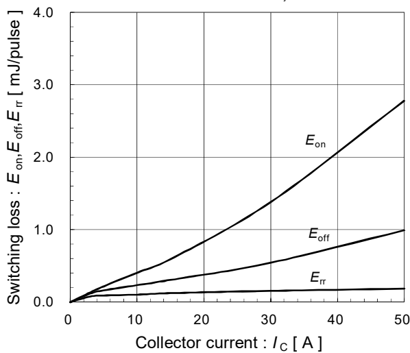
Switching loss vs. Collector current (typ.) V_{DC}=300\text{V}, V_{CC}=15\text{V}, T_{vj}=25^\circ\text{C}
