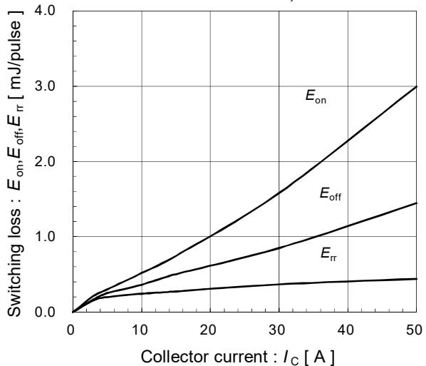
Switching loss vs. collector current (typ.) V_{DC}=300\text{V}, V_{CC}=15\text{V}, T_{vj}=150^\circ\text{C}
