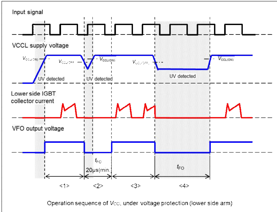
Fig.2-3 Operation sequence of V_{CCL} under voltage protection (lower side arm)
