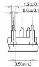
DETAIL D
