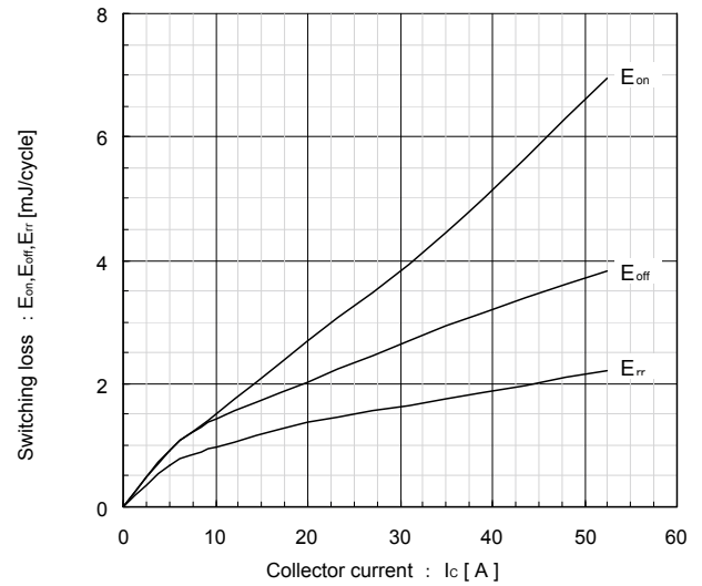
Switching Loss vs. Collector Current (typ.) V_{DC}=600V, V_{CE}=15V, T_J=125^{\circ}C
