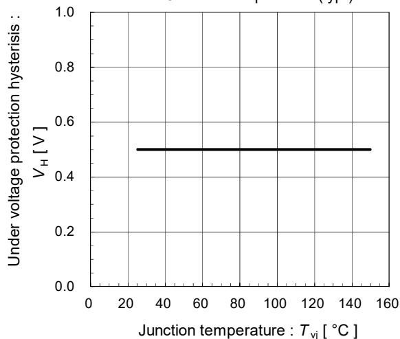
Under voltage protection hysteresis vs. Junction temperature (typ.)
