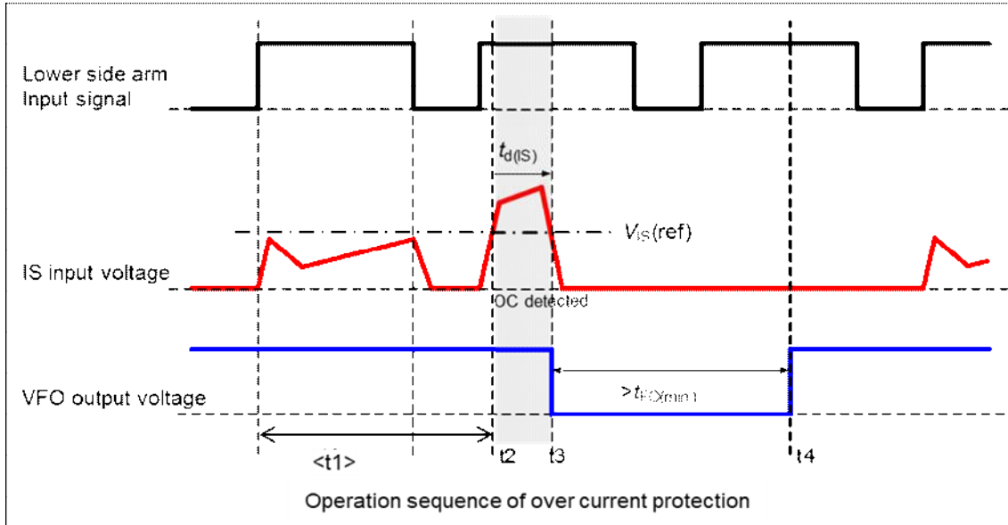
Fig.2-2_Operation_sequence_of over_current_protection
