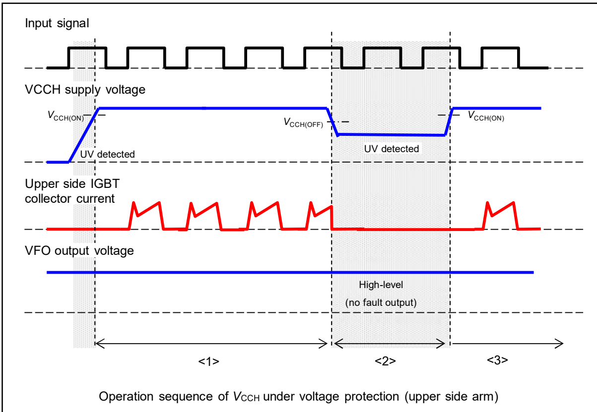
Fig.2-5 Operation sequence of V_{CCH} under voltage protection (upper side arm)
