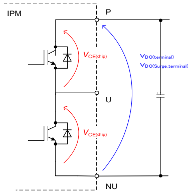
Fig.2-2 Rated voltage
