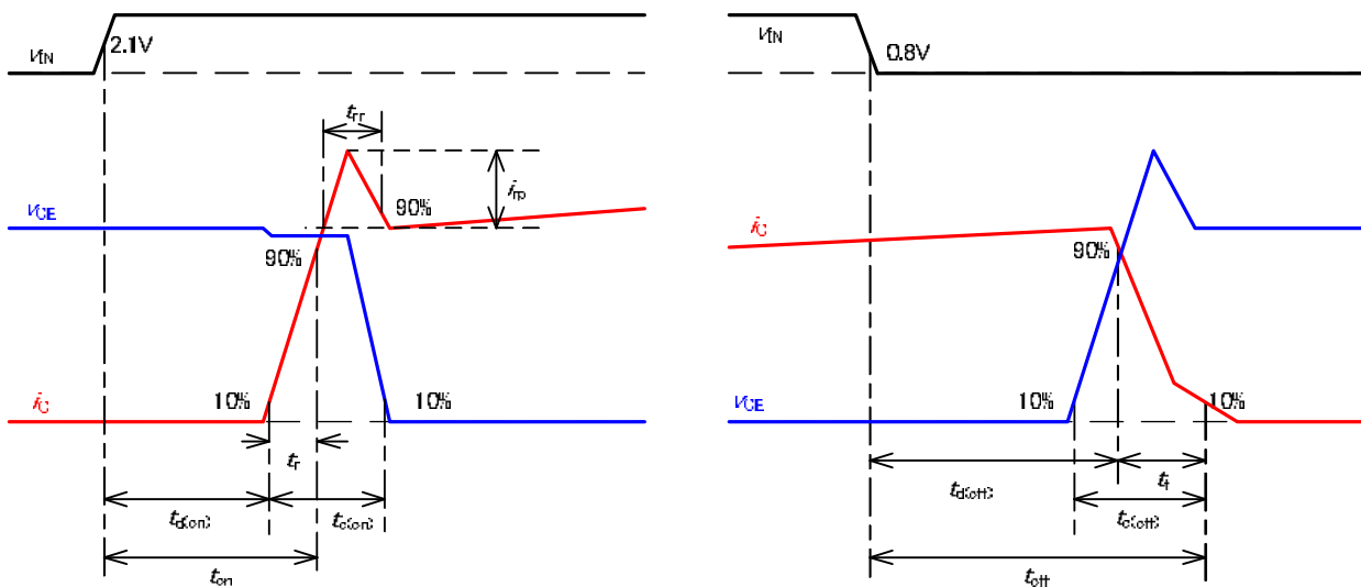
Fig.2-1 Switching waveforms
