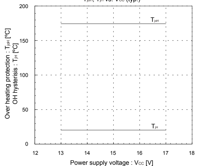
Over heating characteristics T_{J\text{OH}}, T_{JH} vs. V_{CC} (typ.)
