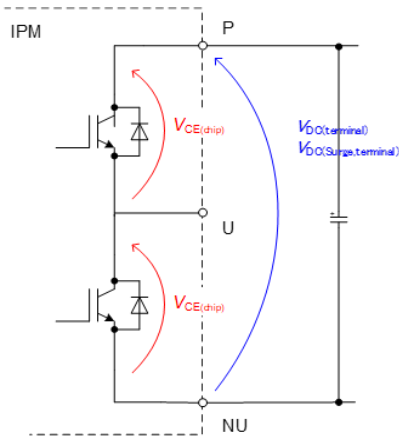
Fig.2-2 Rated Voltage
