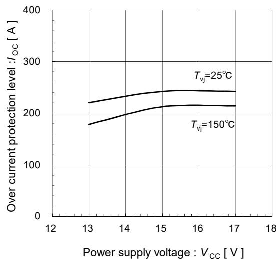
Over current protection vs. Power supply voltage (typ.) V_{DC}=300V
