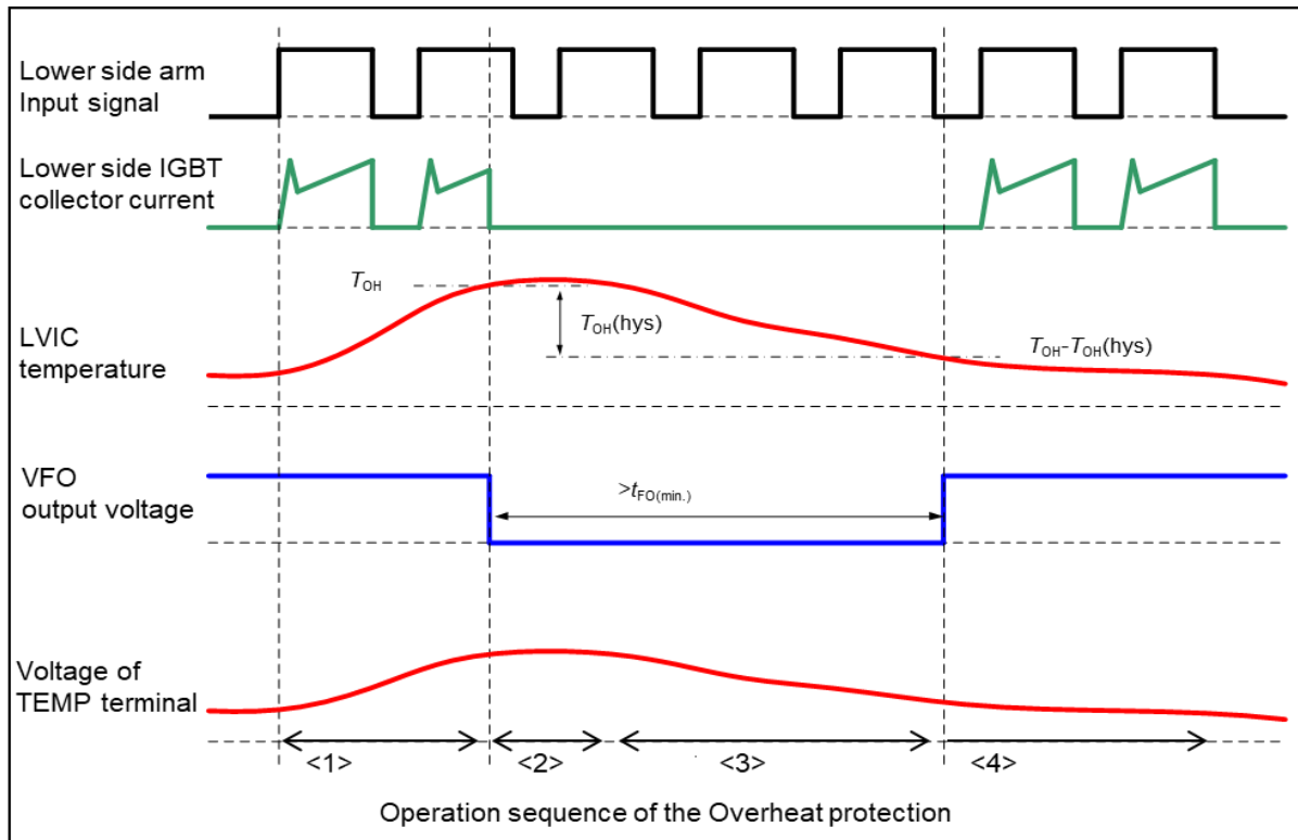
Fig.2-7 Overheat Protection
