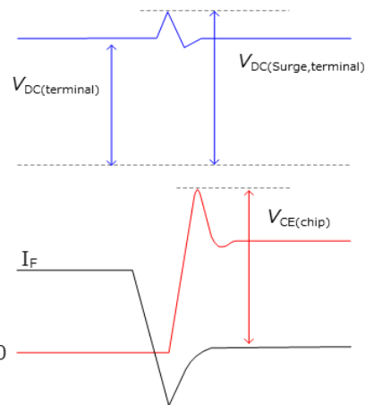
[FWD recovery]
