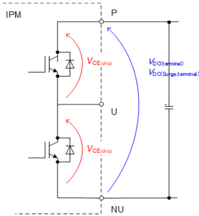
Fig.2-2 Rated Voltage
