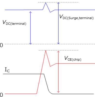
[IGBT turn-off]
