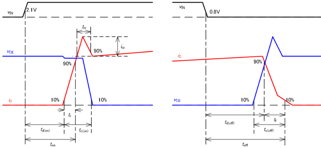
Fig.2-1 Switching waveforms
