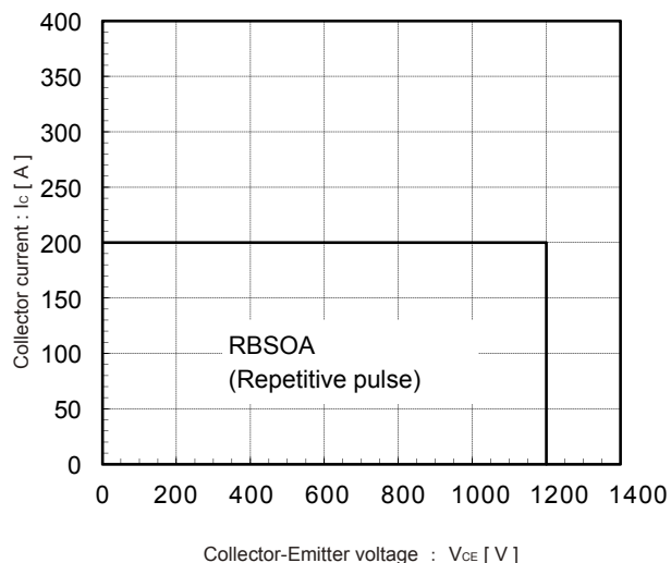
Reversed biased safe operating area V_{CE}=15V, T_J \leq 125^{\circ}C
