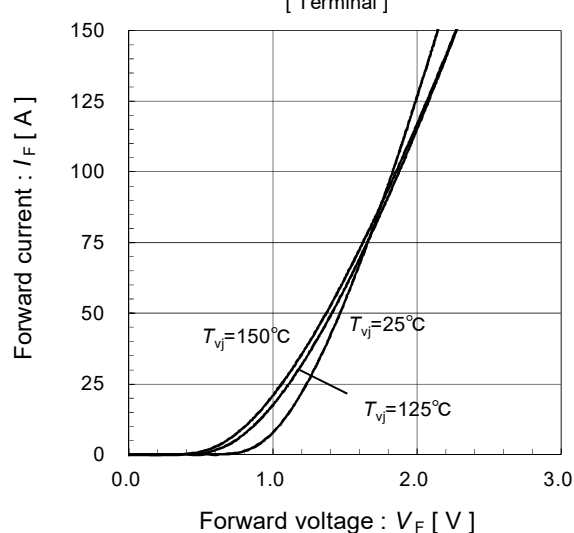
Forward current vs. Forward voltage (typ.)
