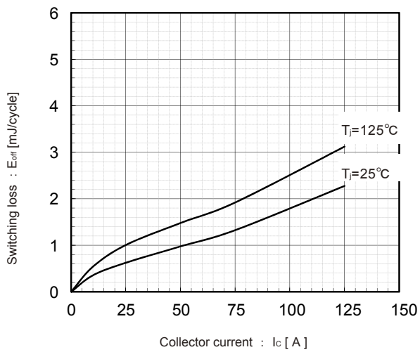
Switching Loss vs. Collector Current (typ.) V_{DC}=300V, V_{CE}=15V
