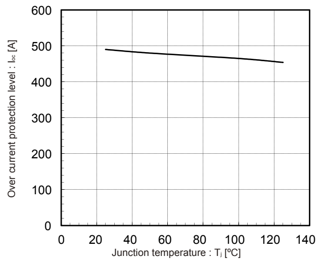
Over current protection vs. Junction temperature (typ.) V_{CE}=15V
