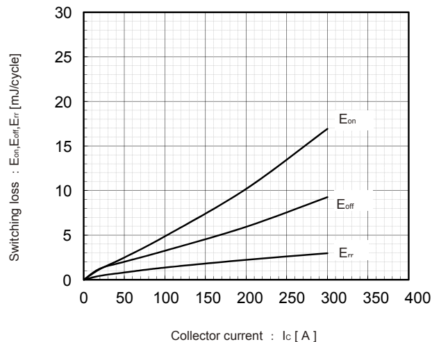
Switching Loss vs. Collector Current (typ.) V_{DC}=300V, V_{CC}=15V, T_J=125^{\circ}C
