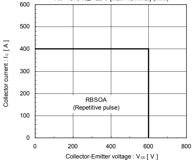
Reversed biased safe operating area V_{CE}=15V , T_J \leq 125^\circ C [Main Terminal] (min.)
