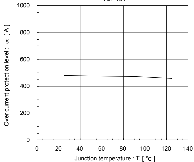
Over current protection vs. Junction temperature (typ.)
