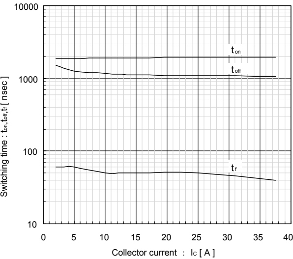
Switching time vs. Collector current (typ.) V_{DC}=600V, V_{CC}=15V, T_J=25^{\circ}C
