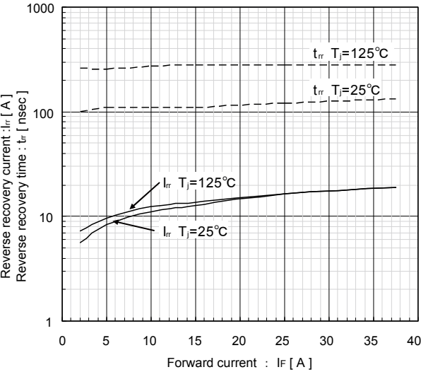
Reverse recovery characteristics (typ.) t_{rr}, I_{rr} vs. I_F
