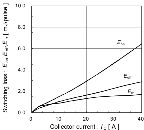
Switching loss vs. Collector current (typ.) V_{DC}=600\text{V}, V_{CC}=15\text{V}, T_{vj}=150^\circ\text{C}
