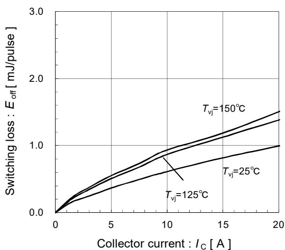
Switching loss vs. Collector current (typ.) V_{DC}=600\text{V}, V_{CC}=15\text{V}, \text{Resistive load}
