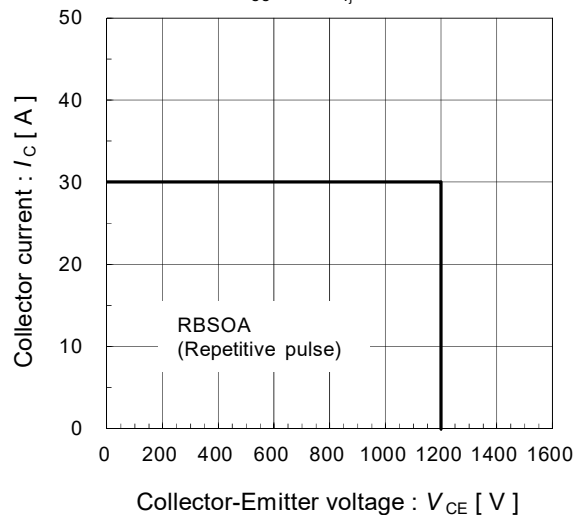
Reversed biased safe operating area V_{CC}=15\text{V}, T_{vj}=150^\circ\text{C}
