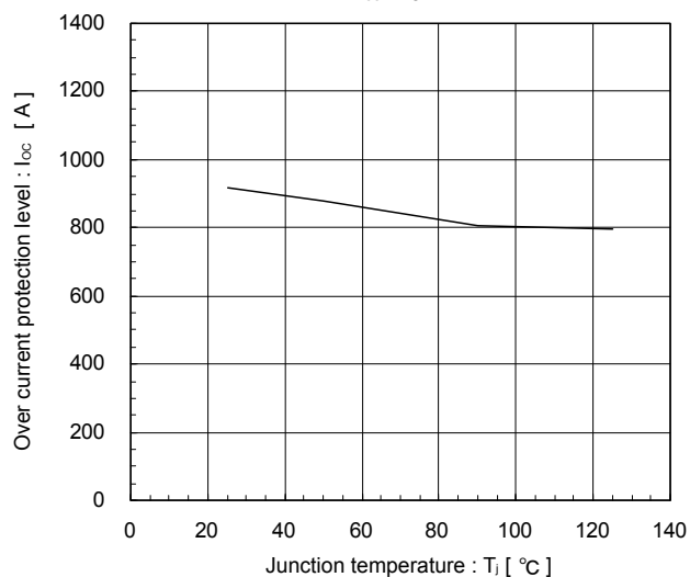
Over current protection vs. Junction temperature (typ.)
