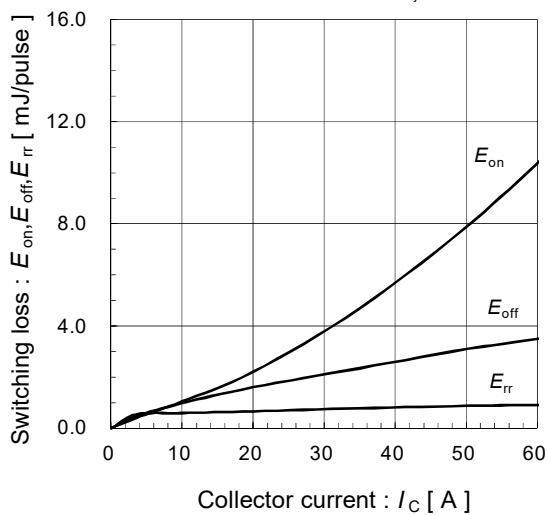
Switching loss vs. Collector current (typ.) V_{DC}=600V, V_{CC}=15V, T_{vj}=25^{\circ}C
