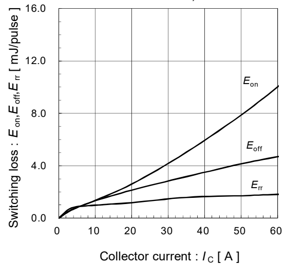
Switching loss vs. Collector current (typ.) V_{DC}=600V, V_{CC}=15V, T_{vj}=125^{\circ}C
