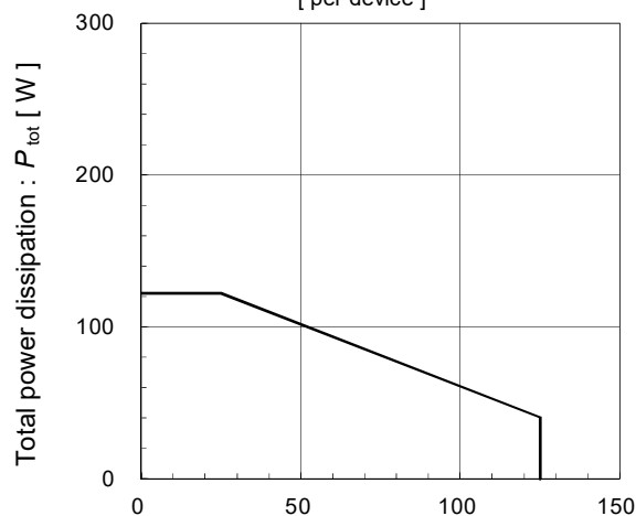
Power derating for FWD (max.) [ per device ]
