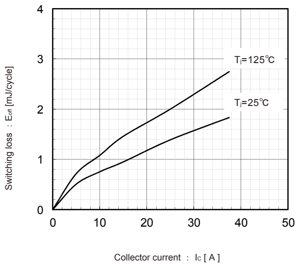
Switching Loss vs. Collector Current (typ.) V_{DC}=600V, V_{CE}=15V
