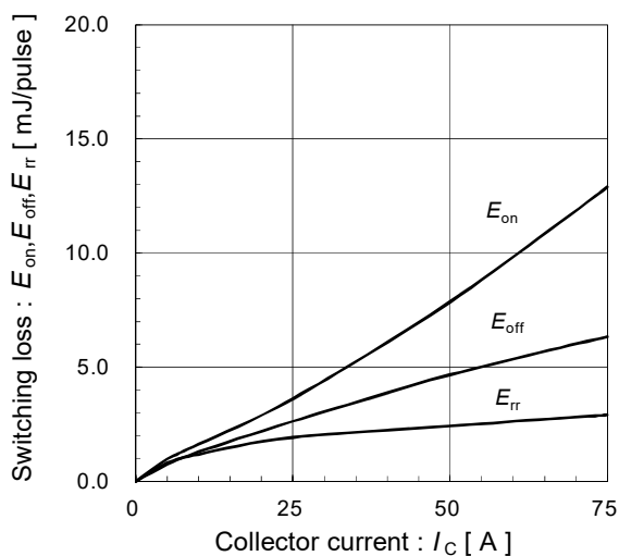
Switching loss vs. Collector current (typ.) V_{DC}=600V, V_{CC}=15V, T_{vj}=150^{\circ}C
