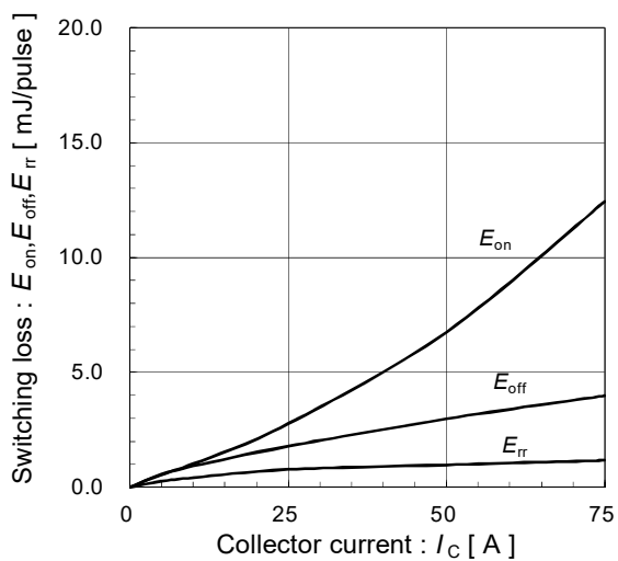
Switching loss vs. Collector current (typ.) V_{DC}=600V, V_{CC}=15V, T_{vj}=25^{\circ}C
