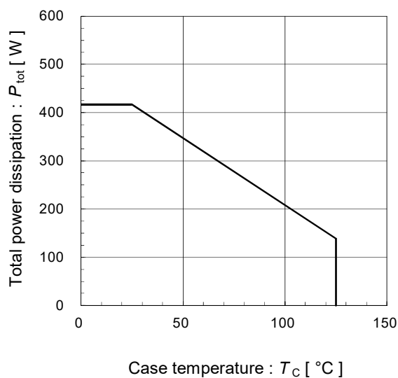
Power derating for IGBT (max.)
