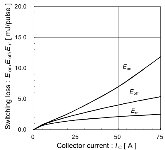
Switching loss vs. Collector current (typ.) V_{DC}=600V, V_{CC}=15V, T_{vj}=125^{\circ}C
