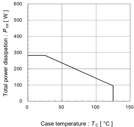
Power derating for FWD (max.)
