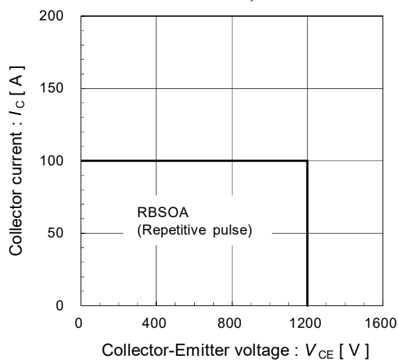
Reversed biased safe operating area (max.)
