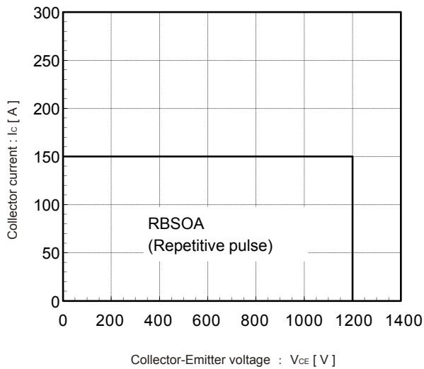
Reversed biased safe operating area V_{CE}=15V, T_J \leq 125^{\circ}C
