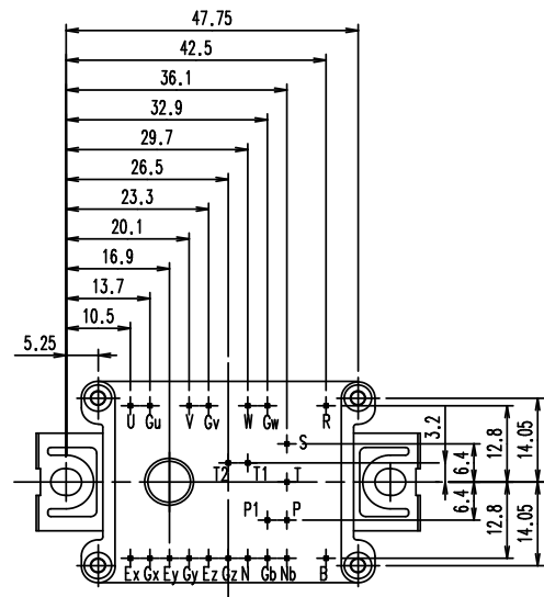
ALL DIMENSION IN THE LEFT FIGURE ARE REFERENCE PIN POSITION TO DESIGNED CENTER OF MODULE \phi \pm 0.7 PIN-BRID SPACING 3.2mm
