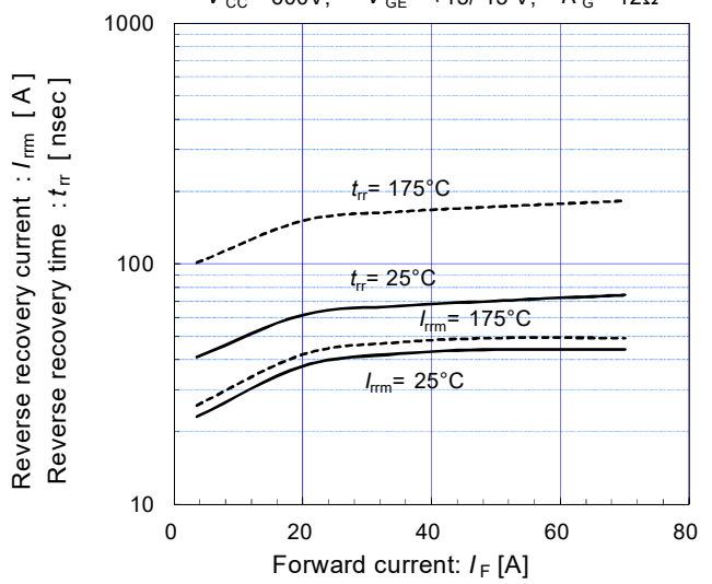
Reverse recovery characteristics (typ.) V_{CC} = 600V, V_{GE} = +15/-15V, R_G = 12\Omega
