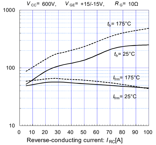
Forward recovery characteristics (typ.)
