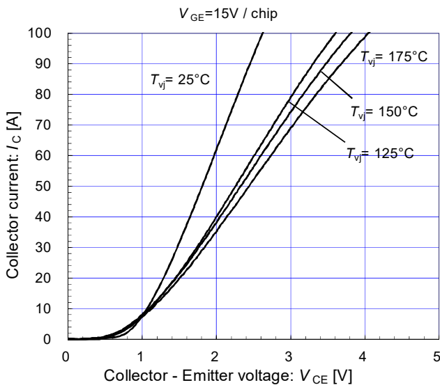
Collector current vs. Collector-Emmitter voltage (typ.)
