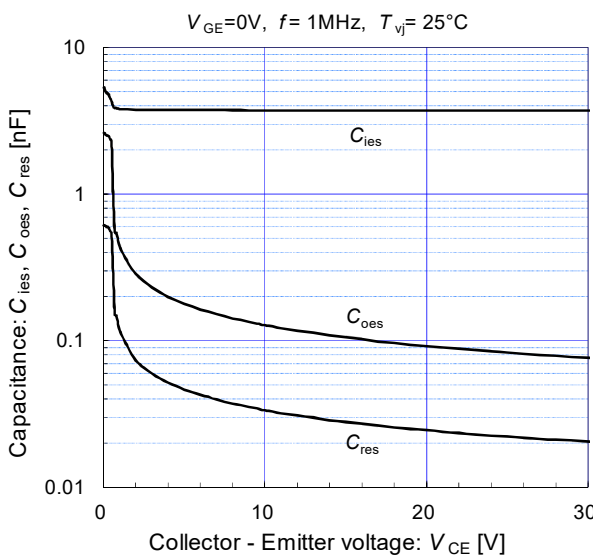
Capacitance vs. Collector-Emittor voltage (typ.)
