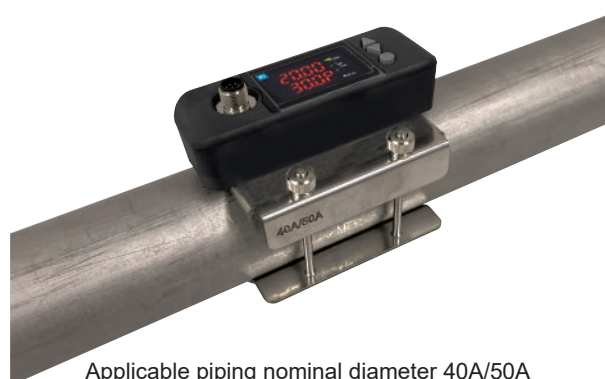
Applicable piping nominal diameter 40A/50A (Type: FSZ40)
