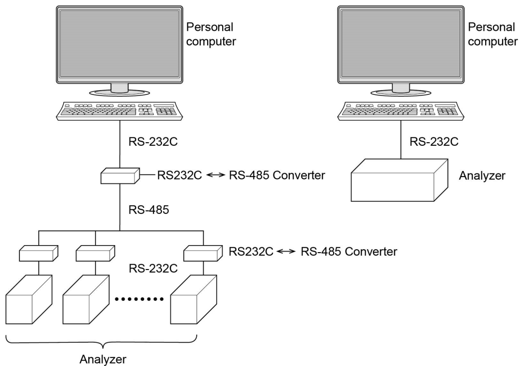
Fig. 1-2 Example of connection with host system
