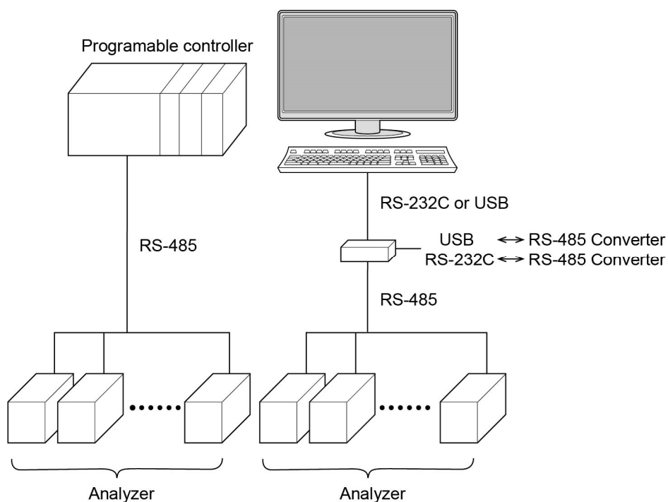
Fig. 1-1 Example of connection with host system
